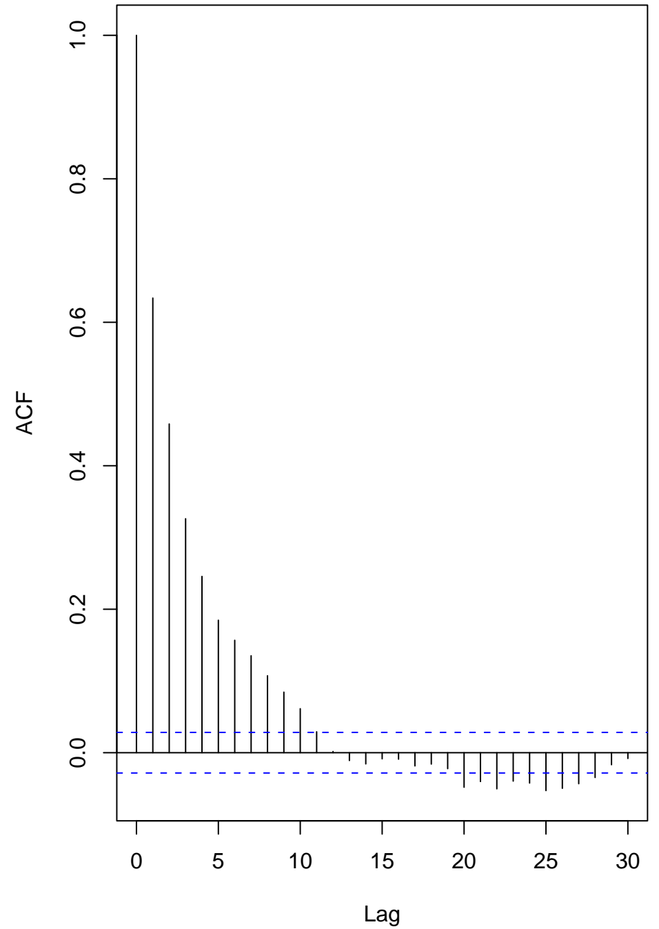
Second Gibbs Sampler
