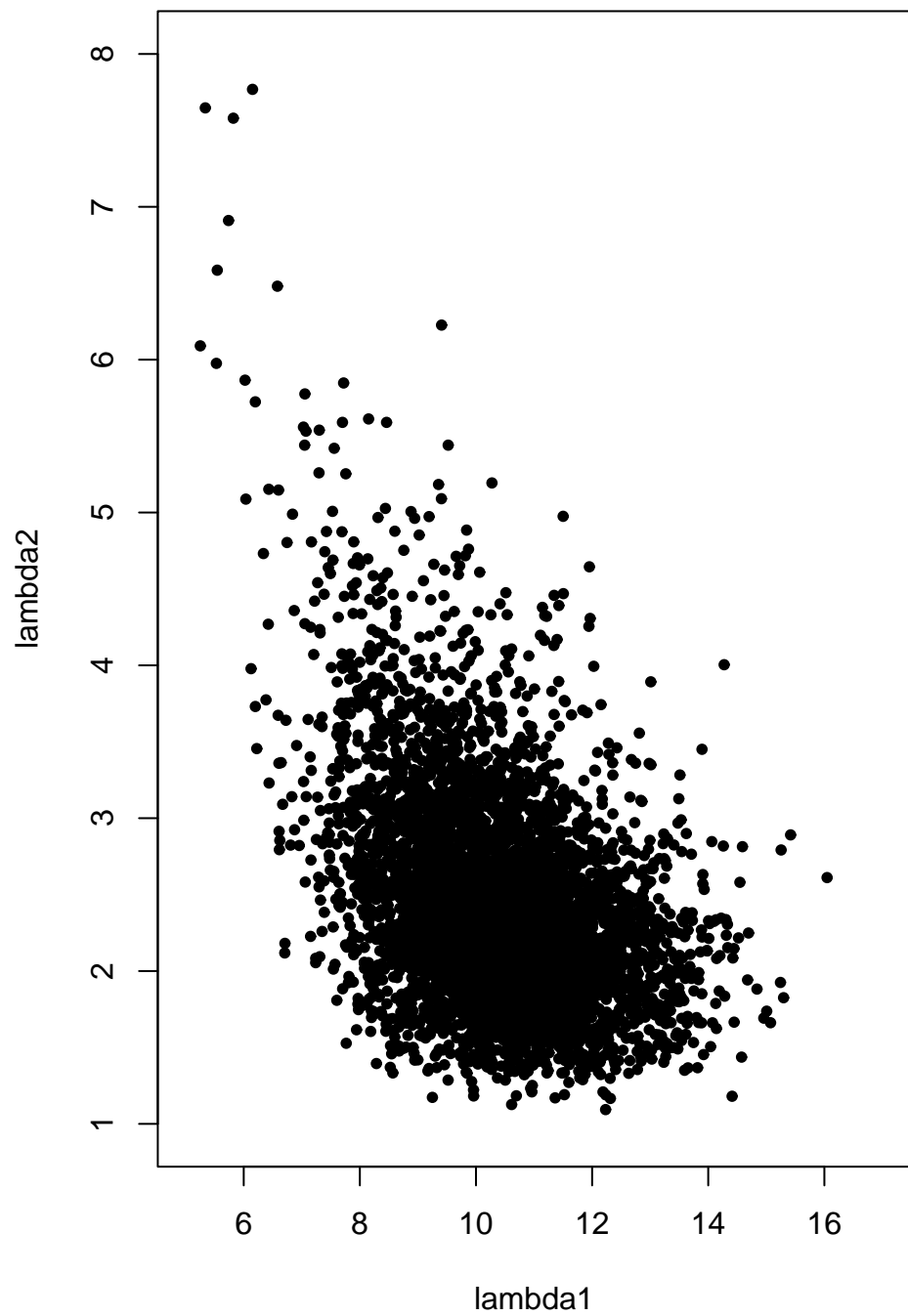
Second Gibbs Sampler
