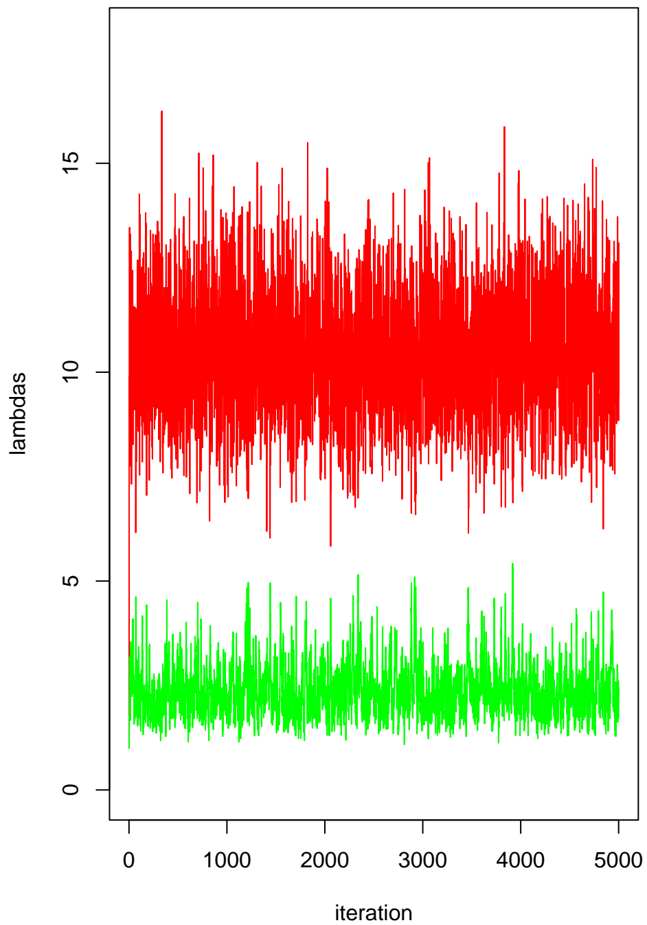
First Gibbs Sampler
