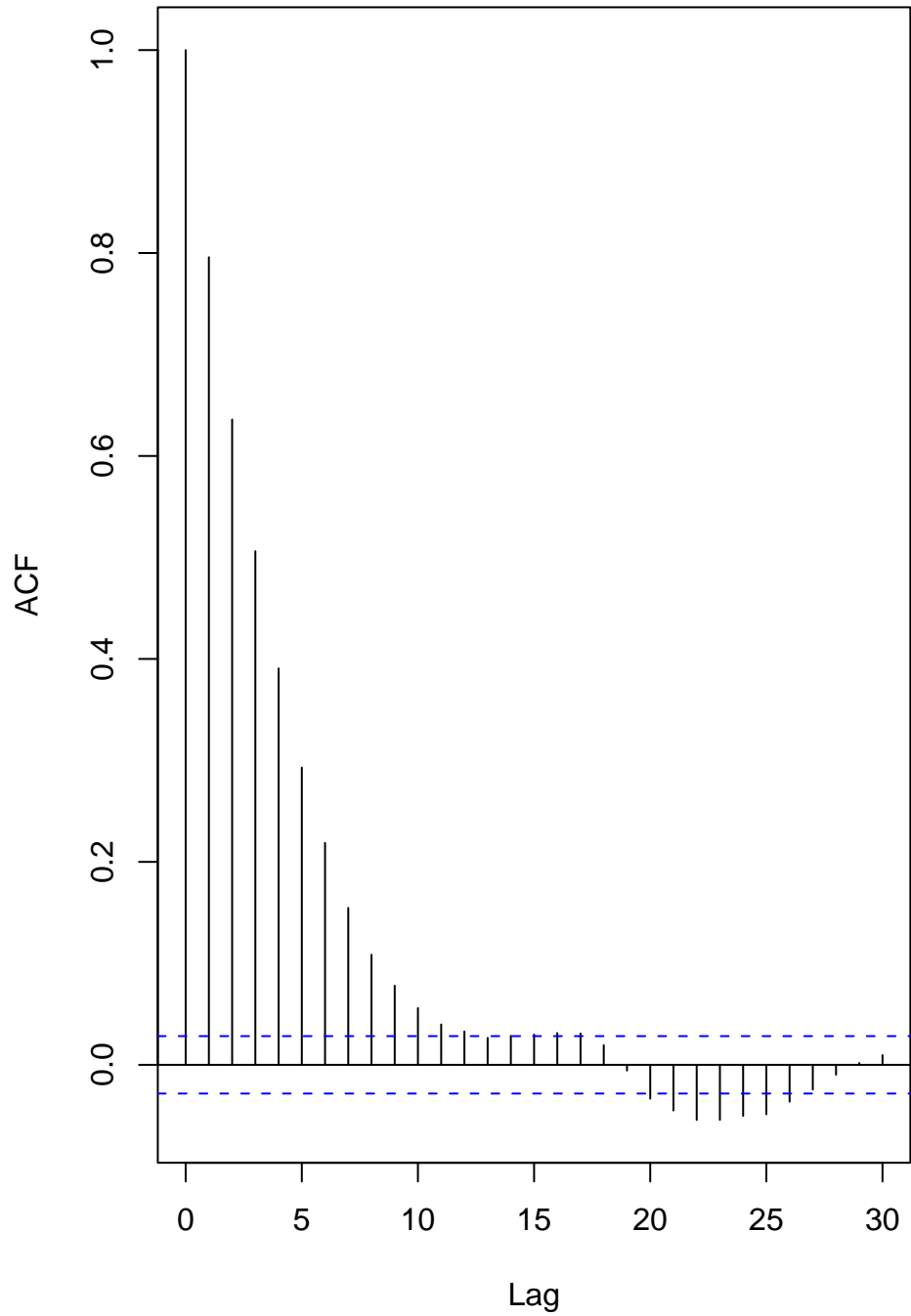
First Gibbs Sampler
