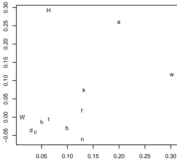
PCA scaled by std. dev. – Unscaled inputs
