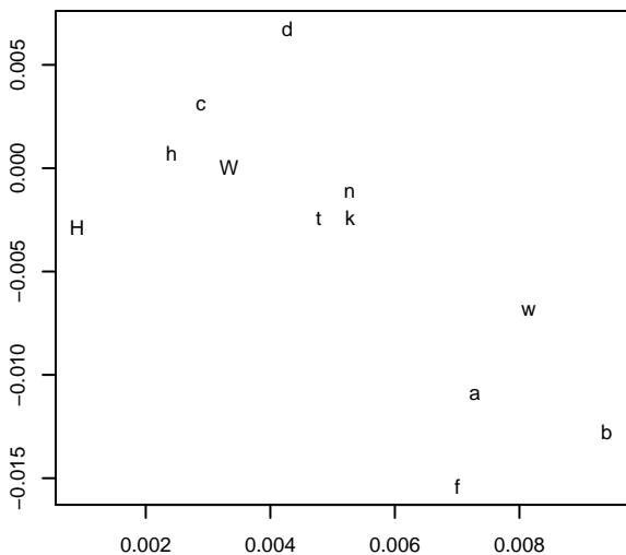
PCA scaled by mean – Unscaled inputs
